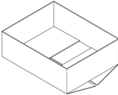
HSCB Half Slotted Carton/Bottom Flap
